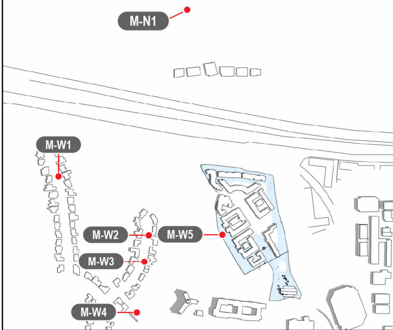
Peninsula Site_Shading_Existing_June 21_1000
