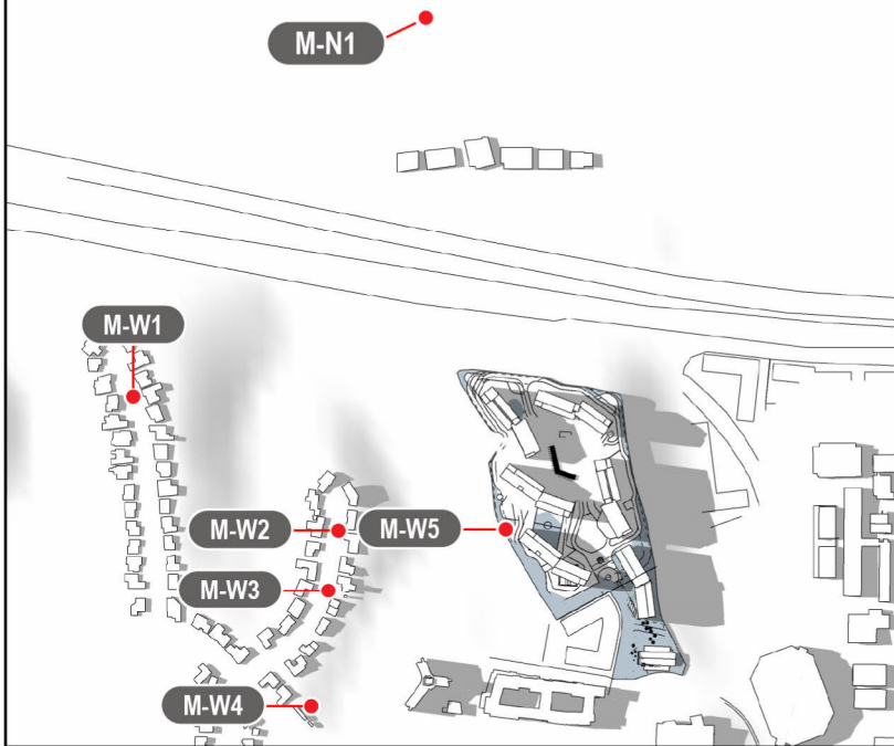
Peninsula Site_Shading_New_June 21_1600
